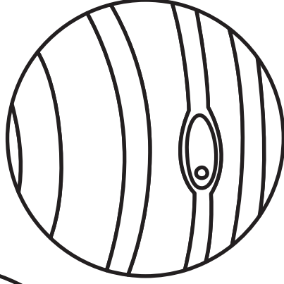
Neptune
